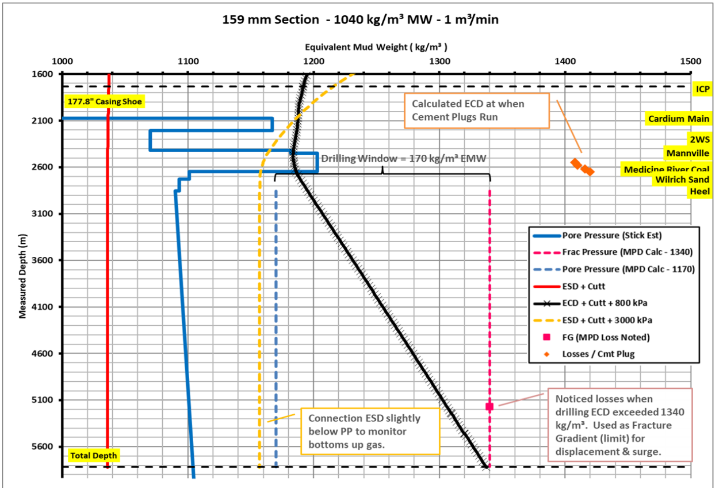
Figure 1: TD well conditions with MPD
